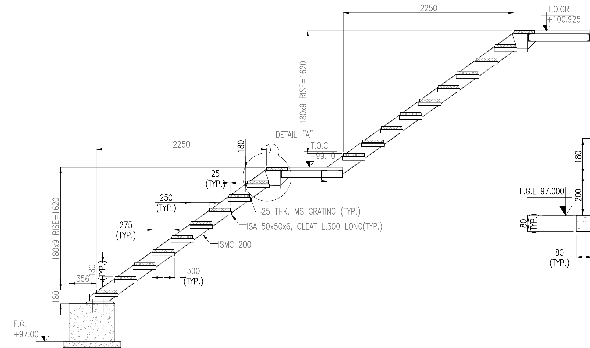
SECTION D-D (SUPPORTS FOR LANDING NOT SHOWN FOR CLARITY) (SCALE 1:40)
