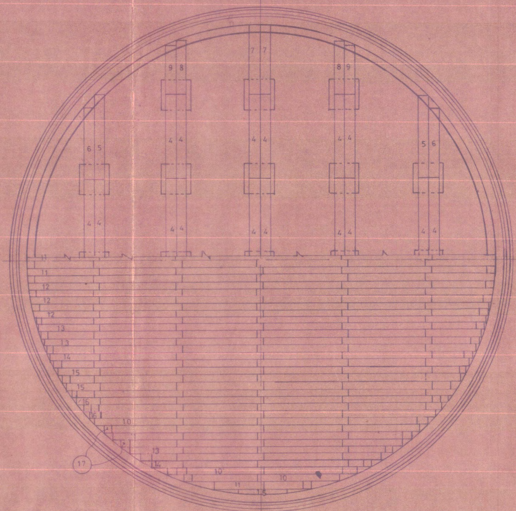
PLAN A-A (NOZZLES NOT SHOWN)
