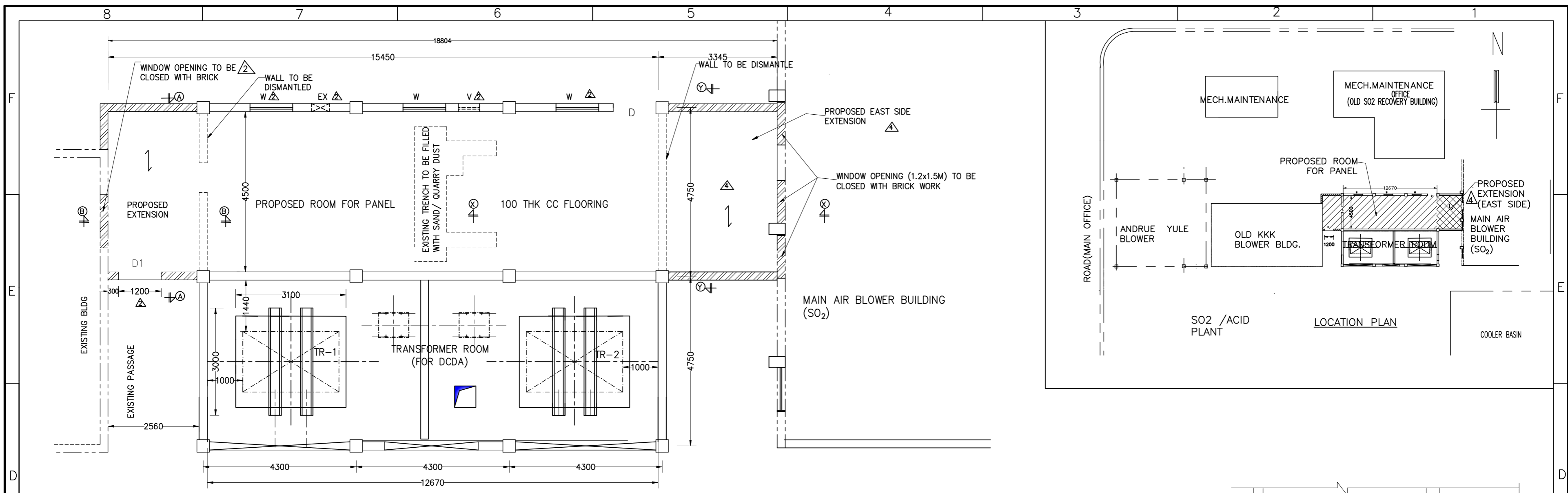
LAYOUT PLAN
