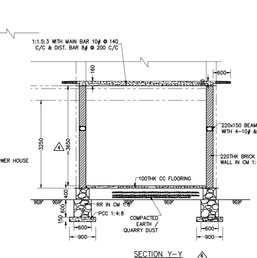
SECTION Y-Y
