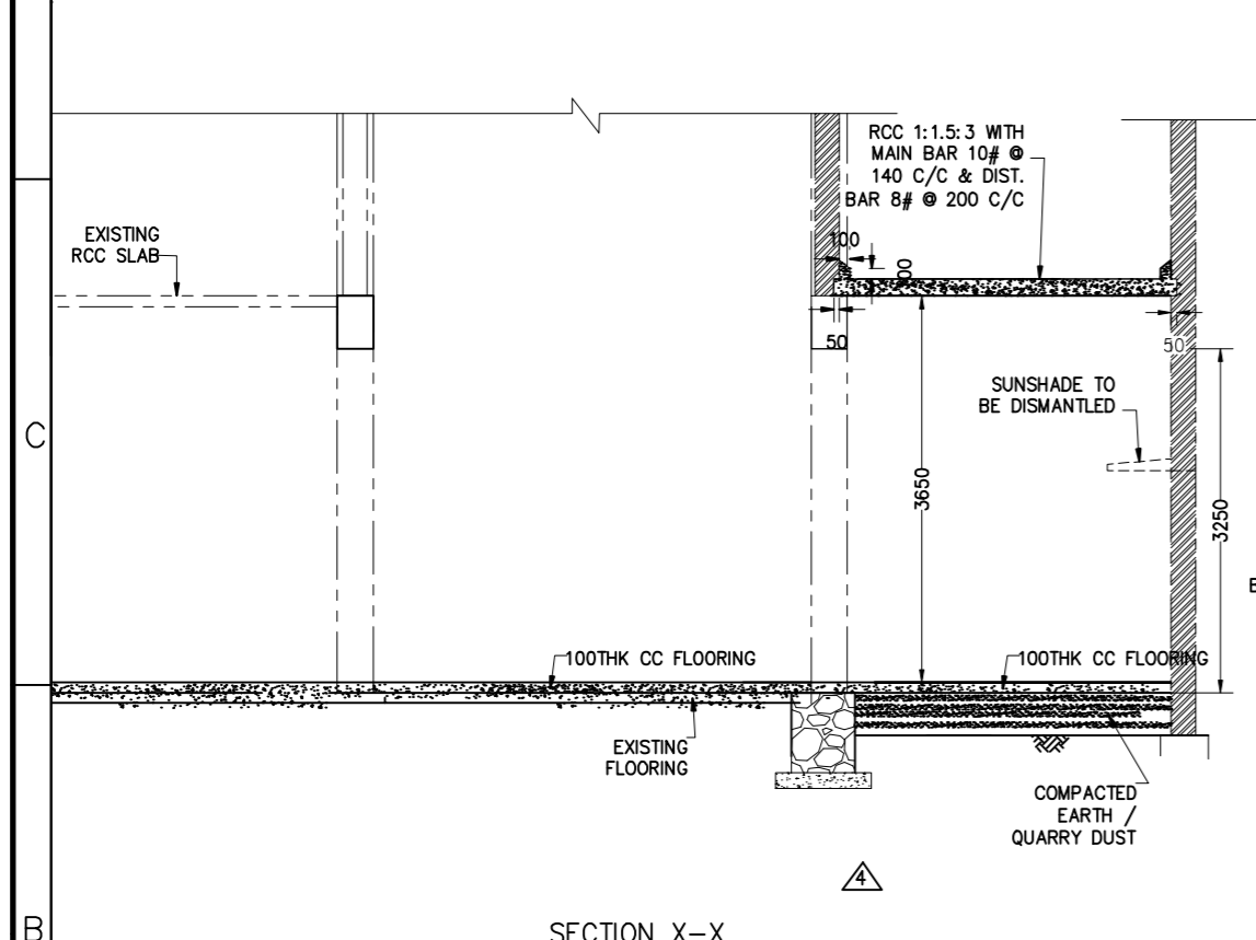
SECTION X-X
